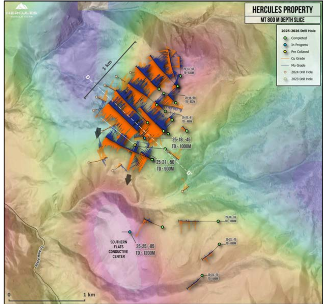
Drill plan showing MT conductivity 800 m below surface. Hotter colours are more conductive. Grade bars for copper (orange) and molybdenum (blue).
