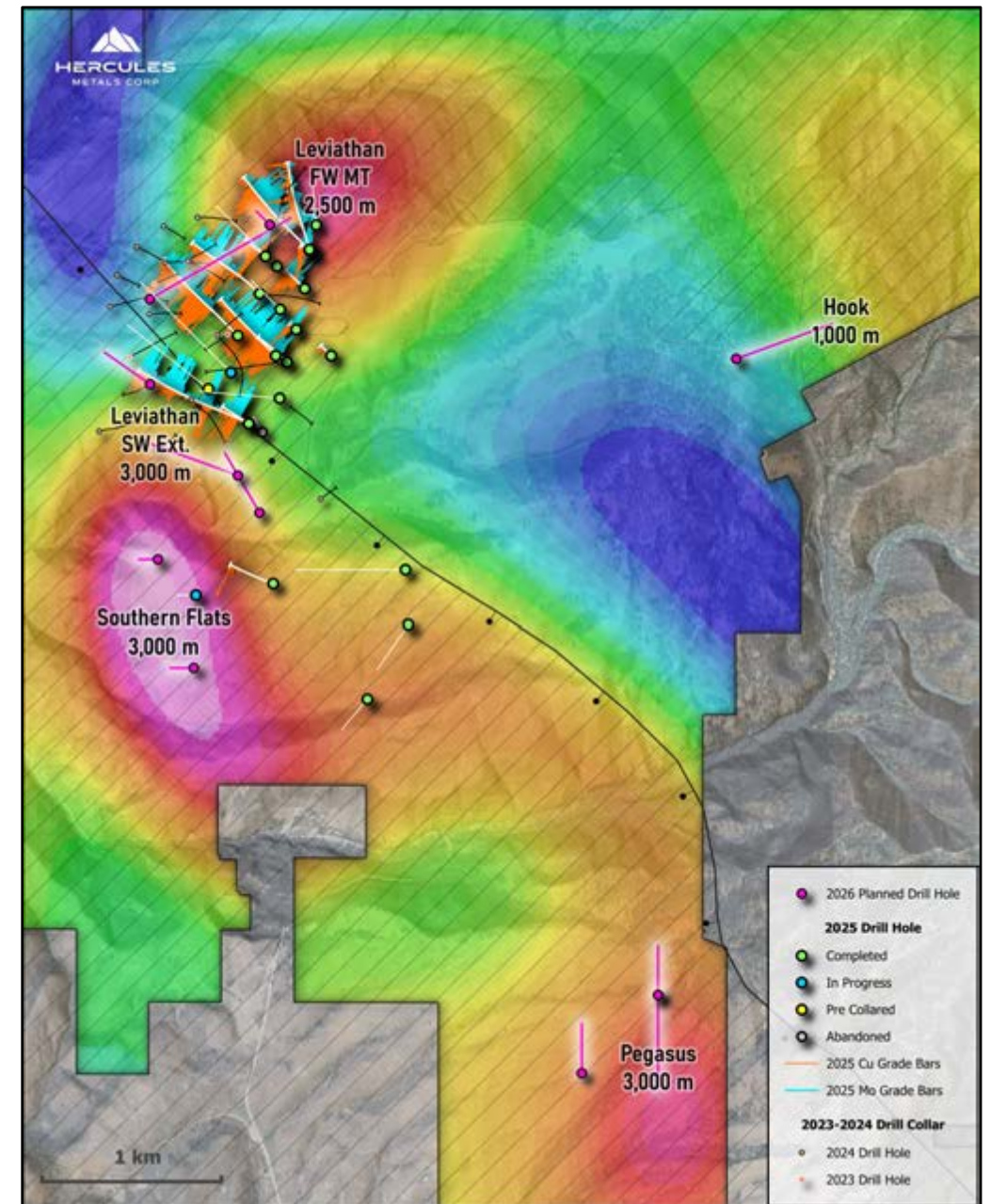
2026 preliminary drill plan showing MT conductivity 800 m below surface. Hotter colours are more conductive than the original Leviathan discovery. Grade bars for copper (orange) and molybdenum (blue).
