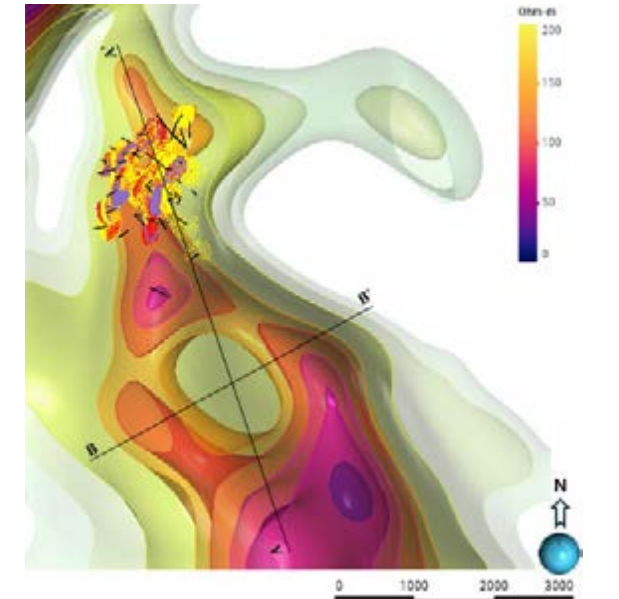
Fig 3: Plan view of Phase I MT anomaly. Modelled copper in the upper part of the image. The anomaly extends for several kilometres southeast of the known mineralization.
