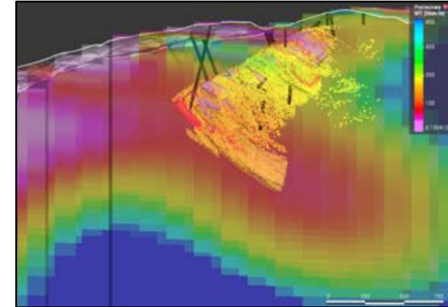
Fig 2: Cross-section looking NE at conductivity model over Leviathan. A SE dipping anomaly (<100 ohm-m) shows a remarkably strong correlation with the southeast dipping copper mineralization in the internal block model.
